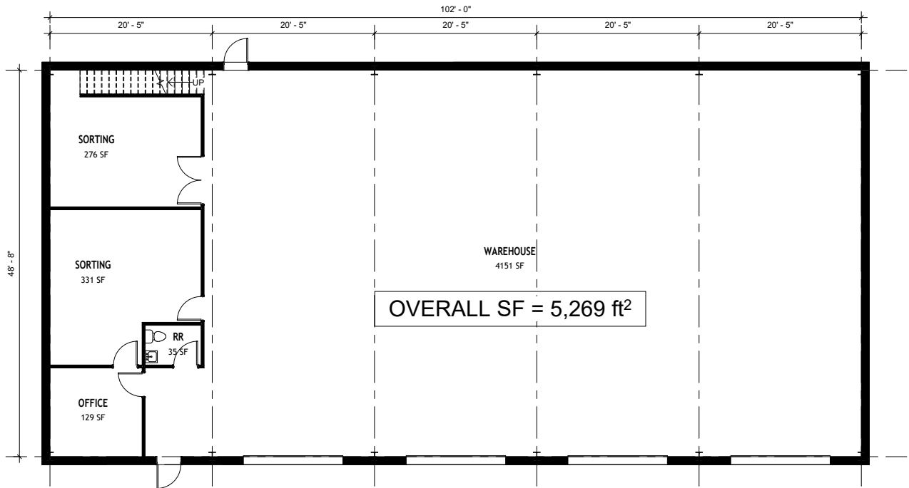
WAREHOUSE B FLOOR PLAN 1/8" = 1'-0"
