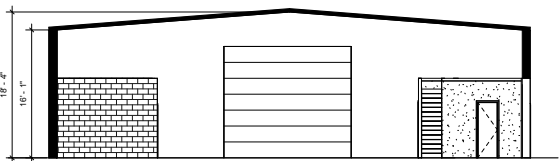
WAREHOUSE C SECTION 1/8" = 1'-0"
